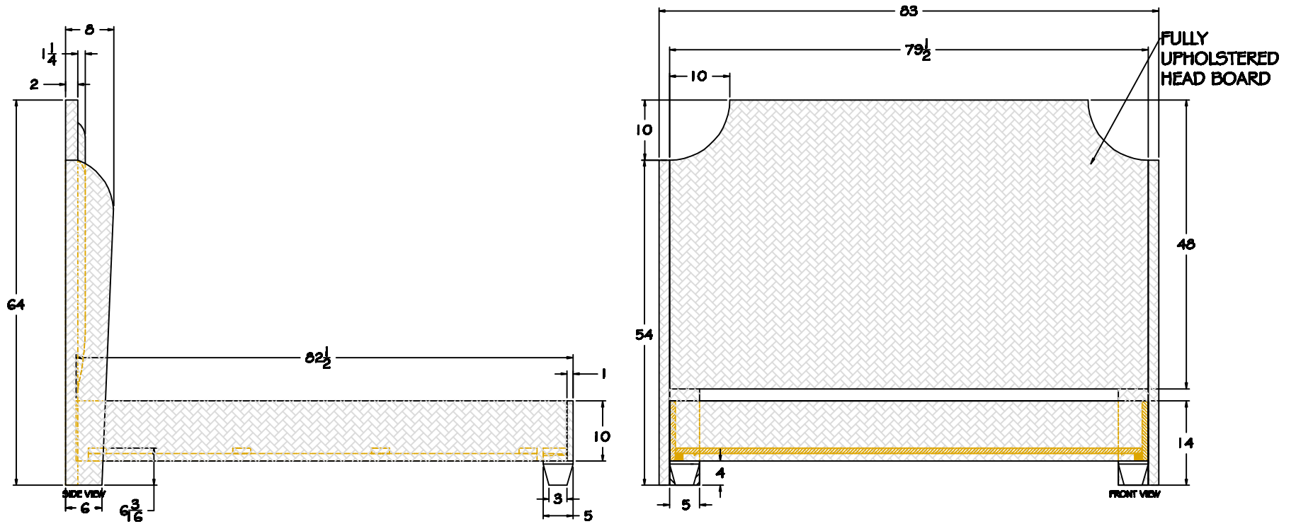
4255-KING WINGED BED, FULLY UPHOLSTERED LORTS
