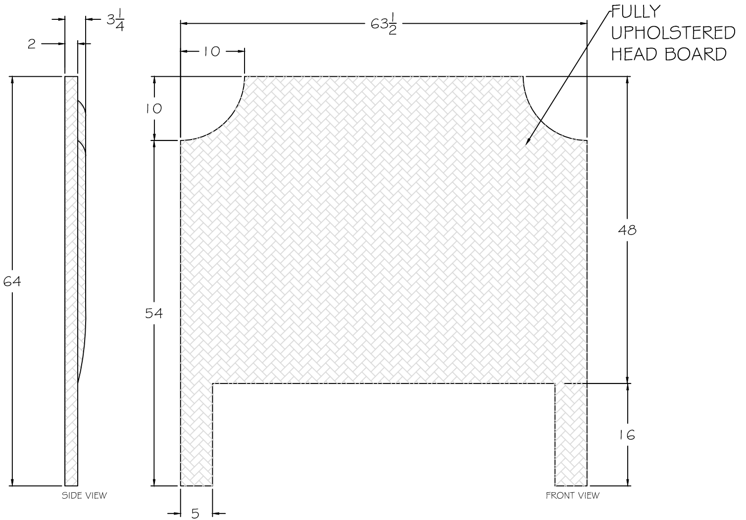
4249 HB- QUEEN HEAD BOARD ONLY, FULLY UPHOLSTERED
