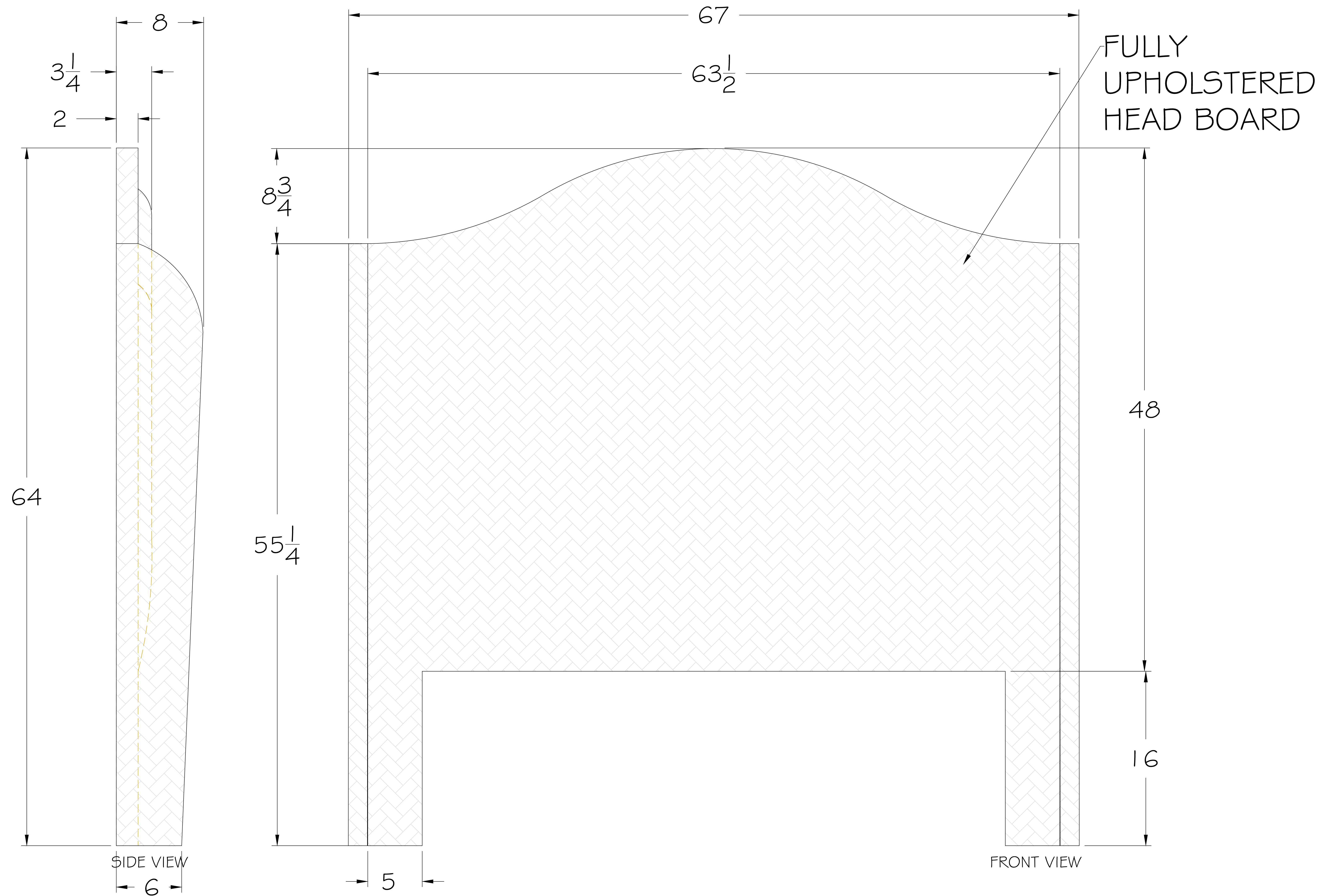
4237 HB- QUEEN WINGED HEAD BOARD ONLY, FULLY UPHOLSTERED
