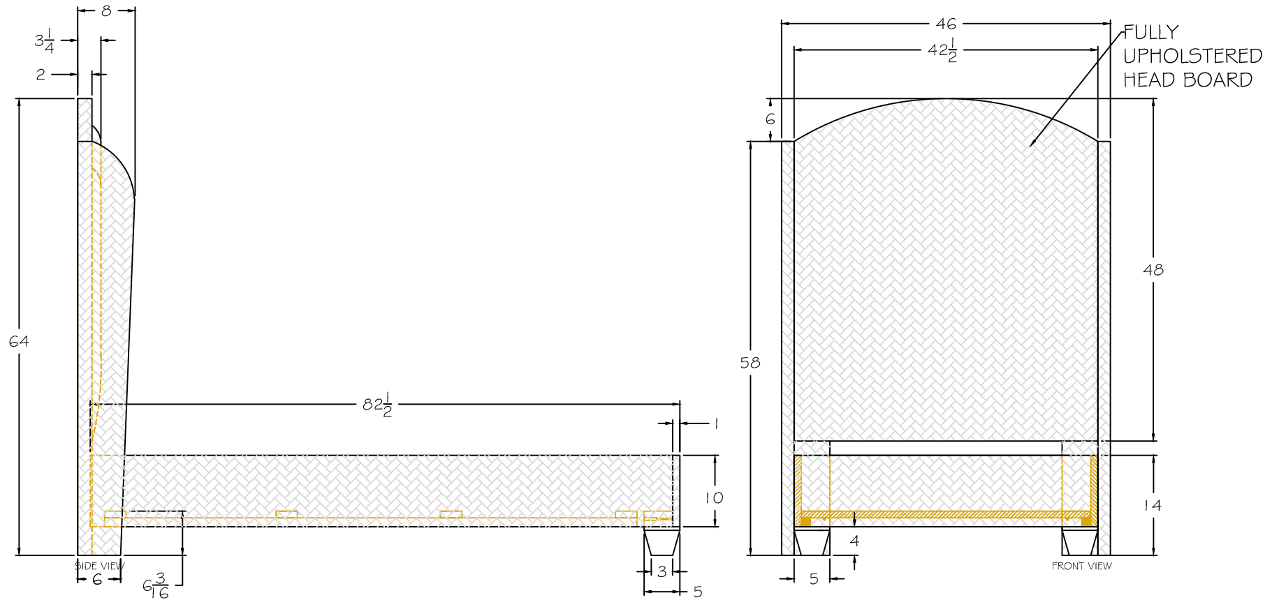
4217- TWIN XL WINGED BED, FULLY UPHOLSTERED
