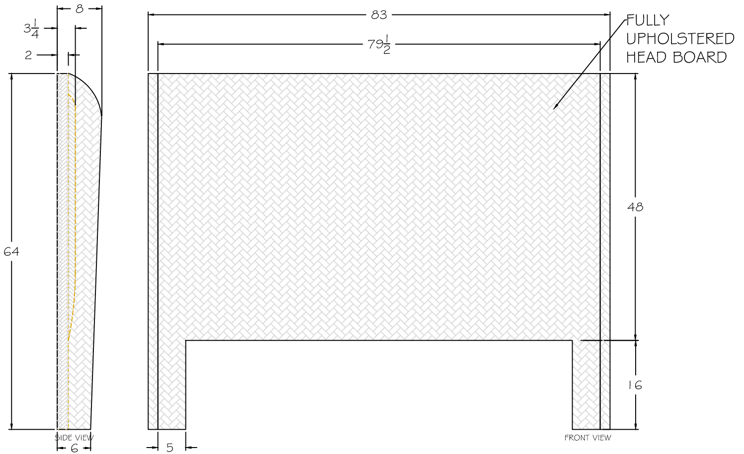
4211 HB- KING WINGED HEAD BOARD ONLY, FULLY UPHOLSTERED
