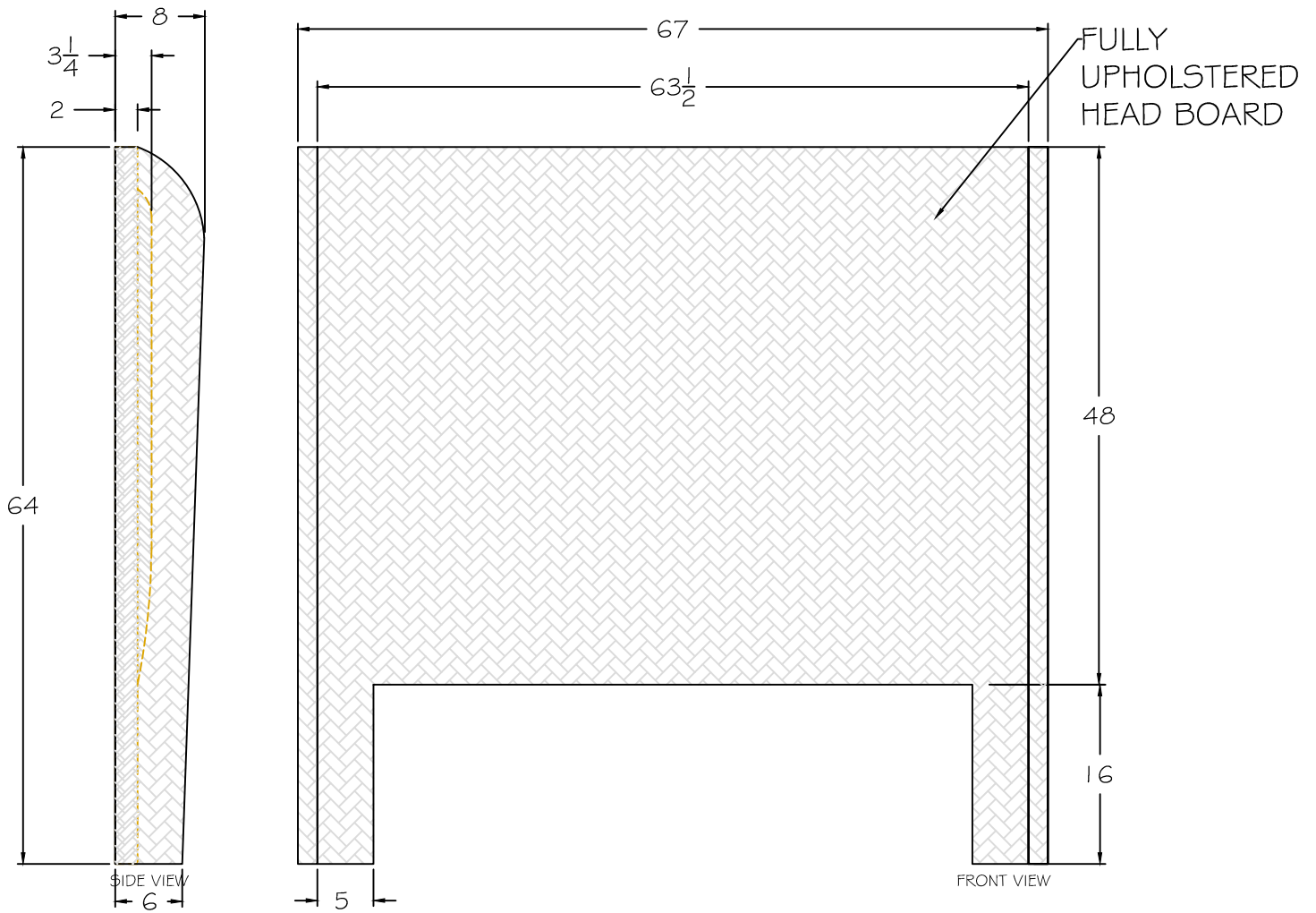
4207 HB- QUEEN WINGED HEAD BOARD ONLY, FULLY UPHOLSTERED
