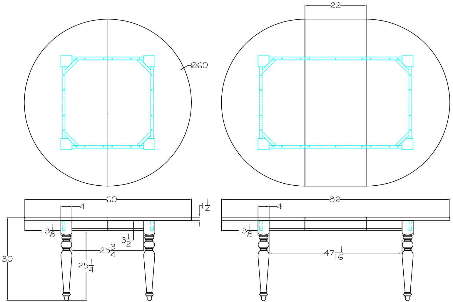
7560L-Dining Table- 60 ROUND X 30H_W/22" LEAF
