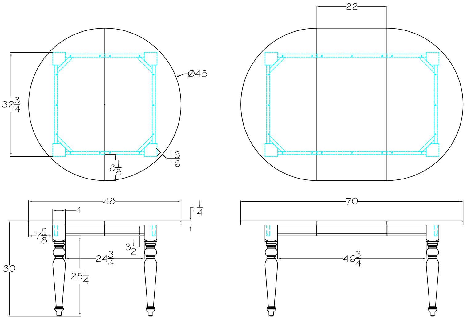
7548L-Dining Table- 48 ROUND X 30H_W/22" LEAF
