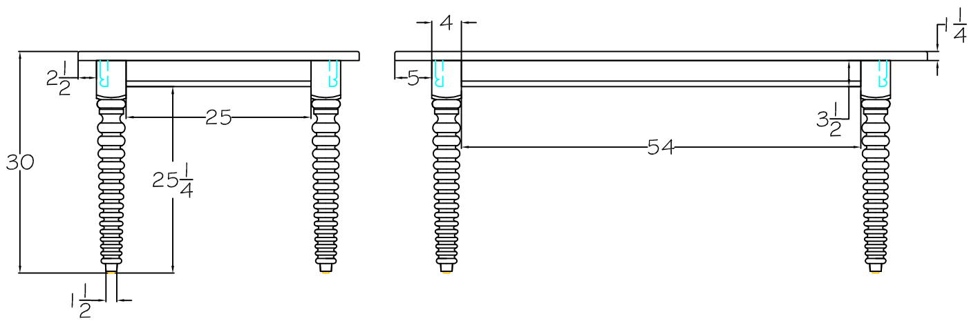
7472-Dining Table- 72W X 38D X 30H
