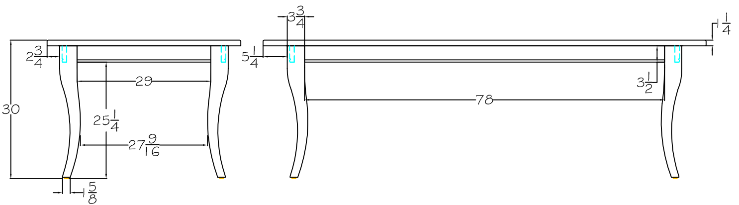
7396-Dining Table- 96W X 42D X 30H
