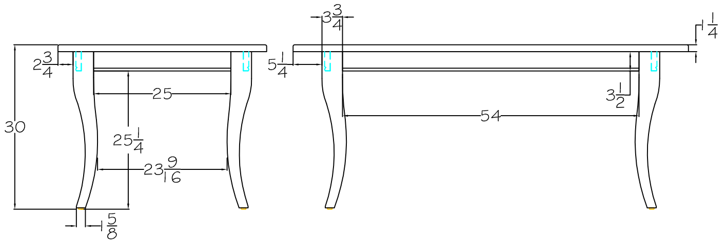
7372-Dining Table- 72W X 38D X 30H
