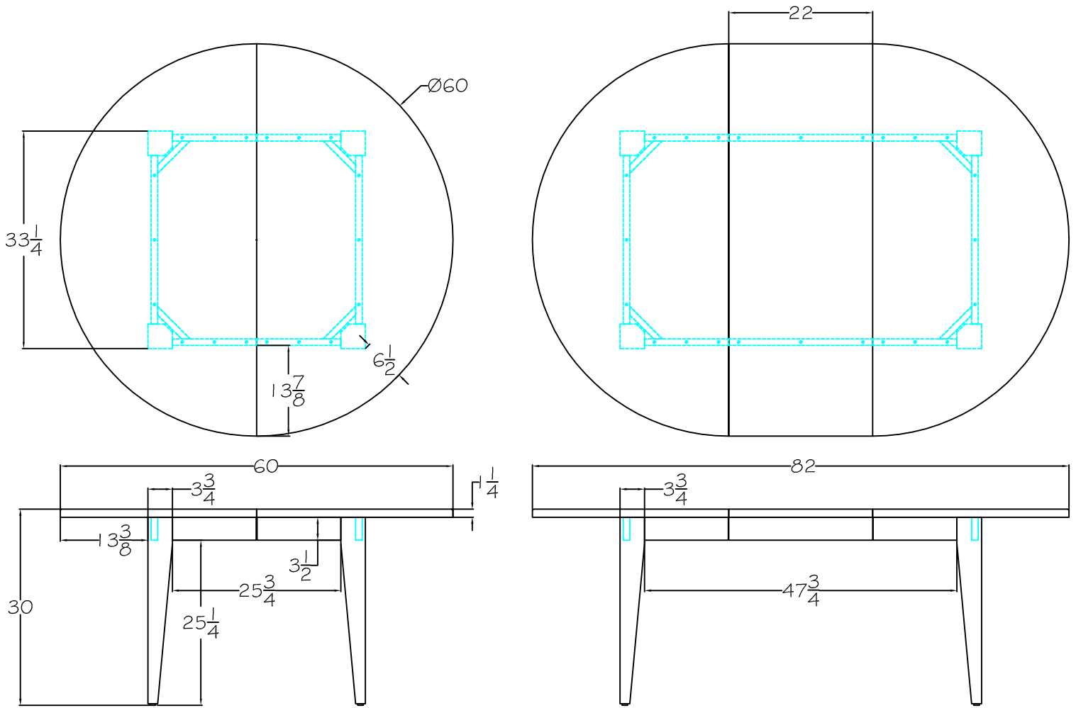
7260L-Dining Table- 60 ROUND X 30H_W/22" LEAF
