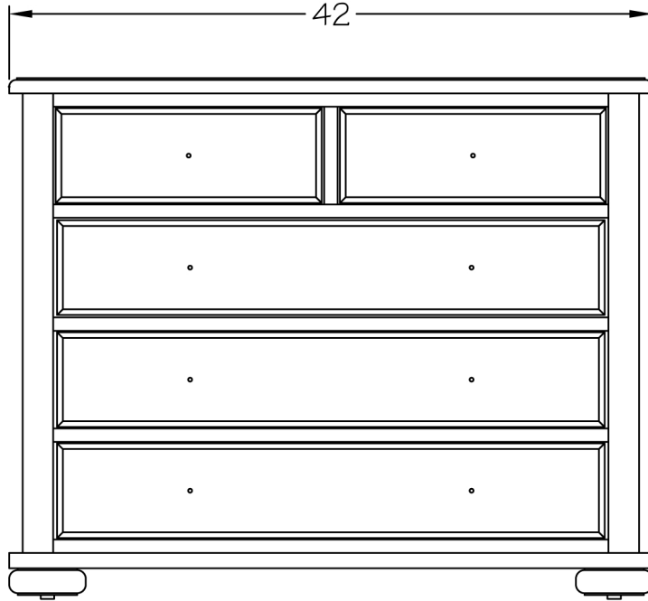
7117 5-DRAWER CHEST
