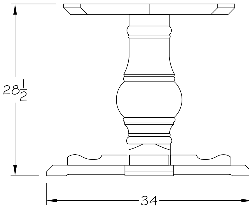
5217-Pedestal Table Base
