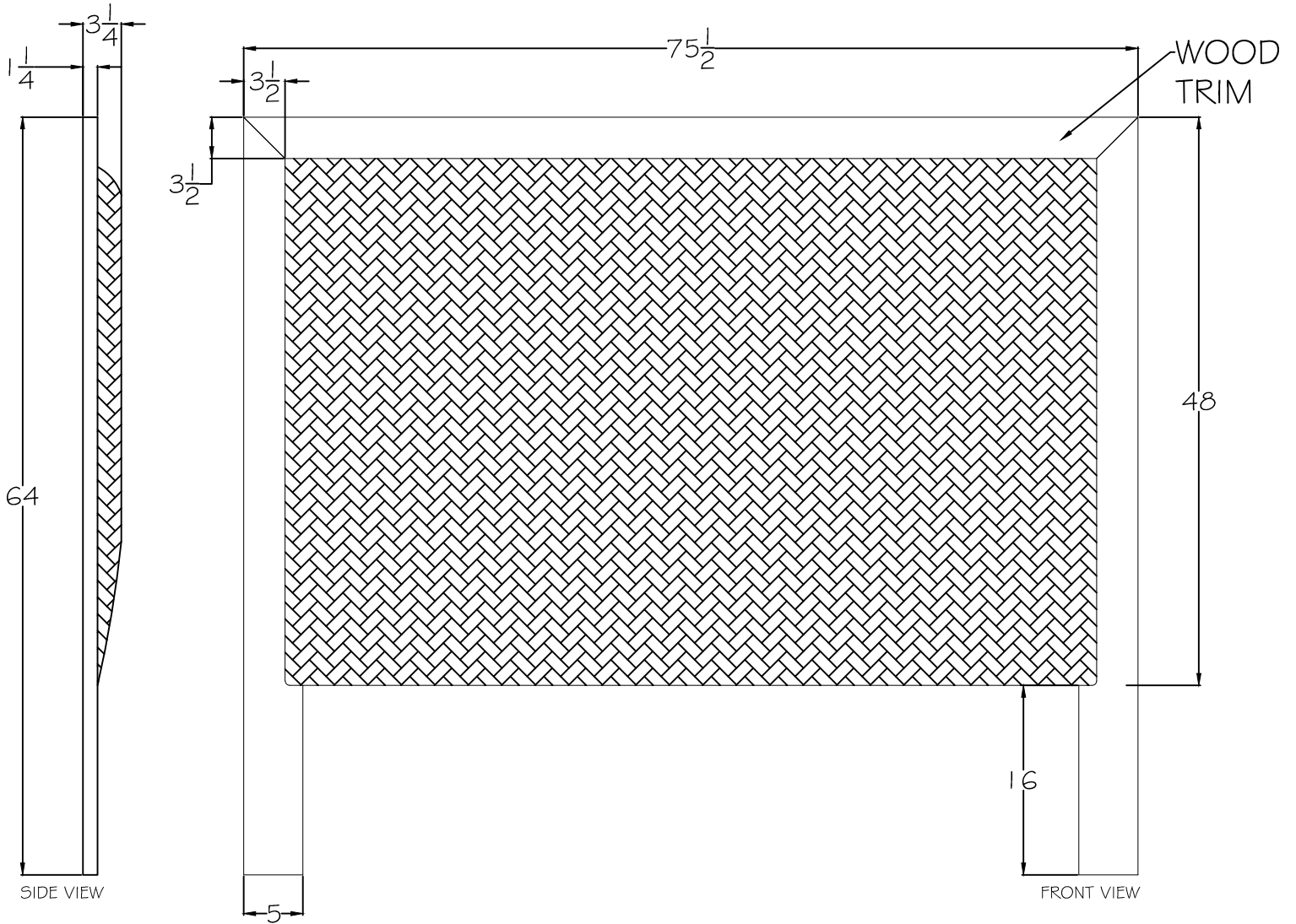
4087 HB- CAL-KING HEAD BOARD ONLY, UPHOLSTERED, WITH WOOD TRIM
