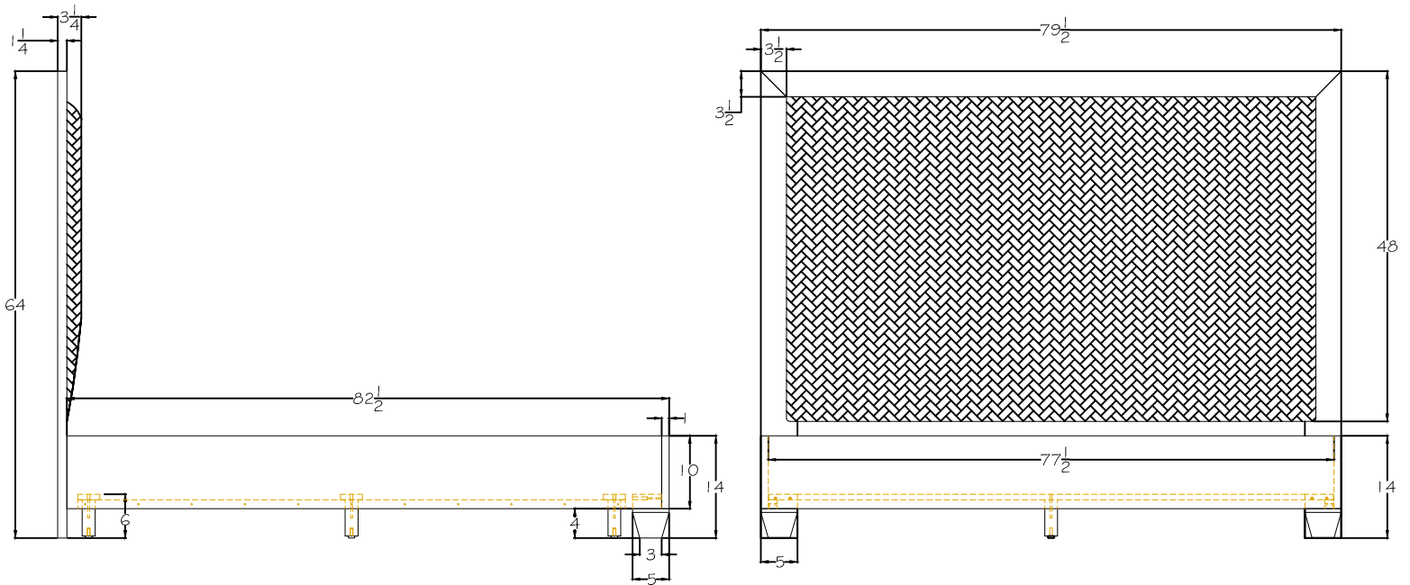
4085- KING BED UPHOLSTERED, WITH WOOD TRIM
