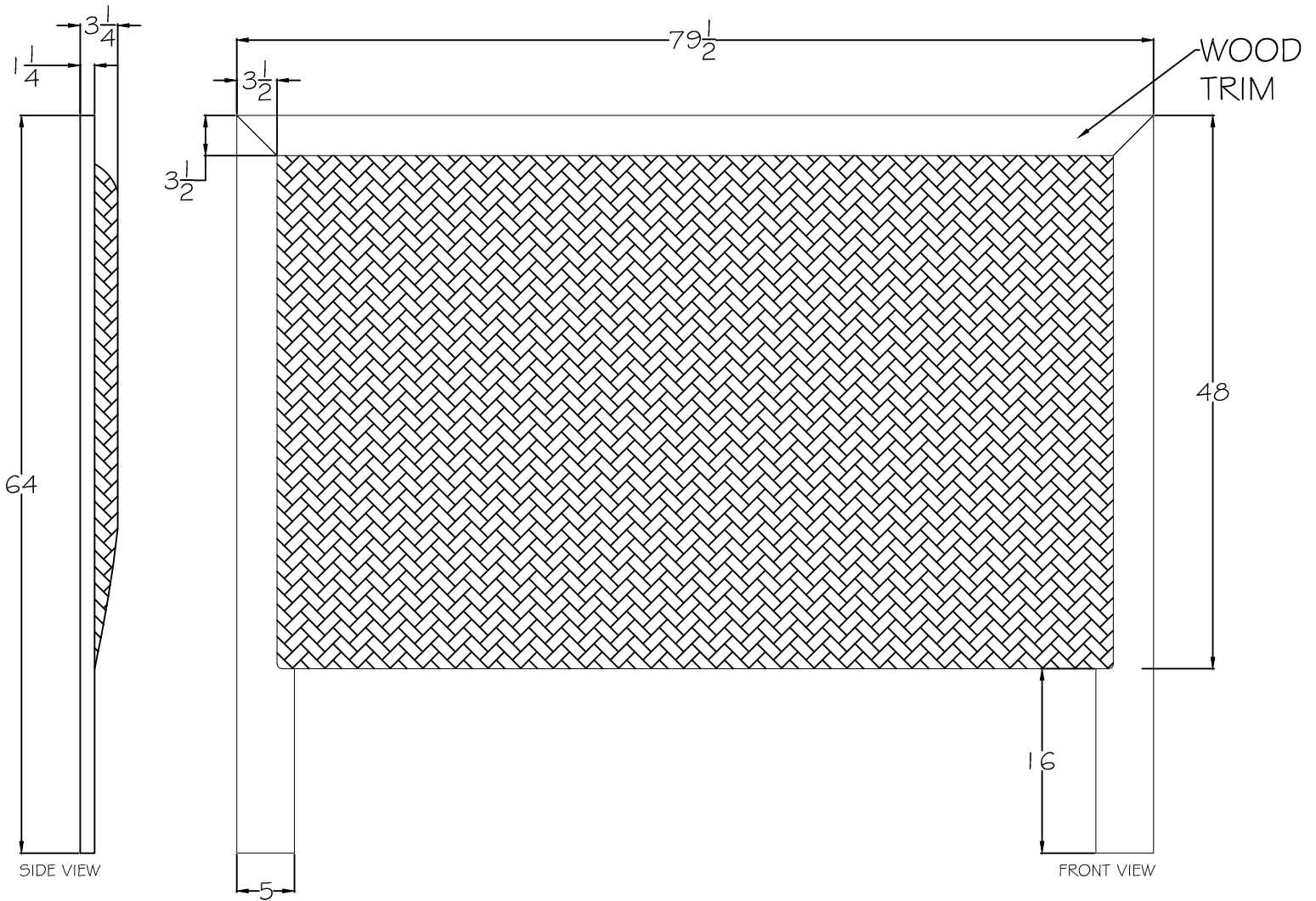
4085 HB- KING HEAD BOARD ONLY, UPHOLSTERED, WITH WOOD TRIM
