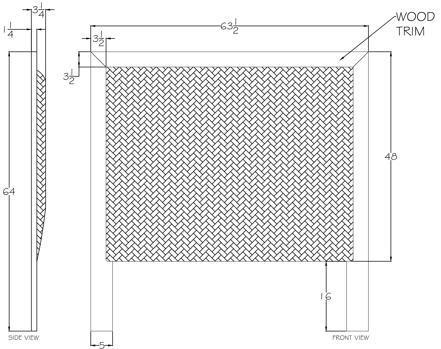
4083 HB- QUEEN HEAD BOARD ONLY, UPHOLSTERED, WITH WOOD TRIM
